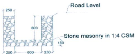
Drain Type - II
