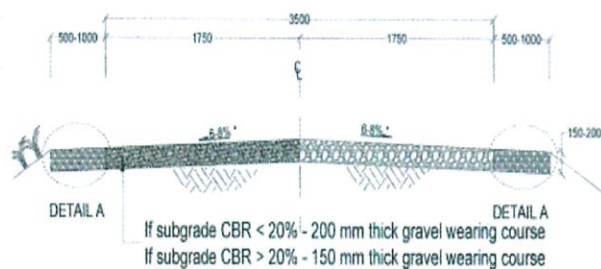
SECTION - 1 GRAVEL SURFACE PAVEMENT
