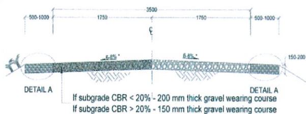
SECTION - 1 GRAVEL SURFACE PAVEMENT
