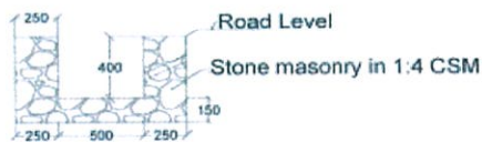
Drain Type - I
